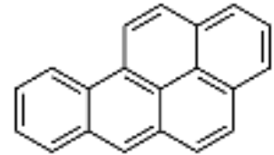
Benzo-a-pyrene
